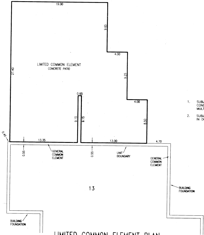
LIMITED COMMON ELEMENT PLAN (PERTAINING TO UNIT 13) SCALE: 1"=5'
